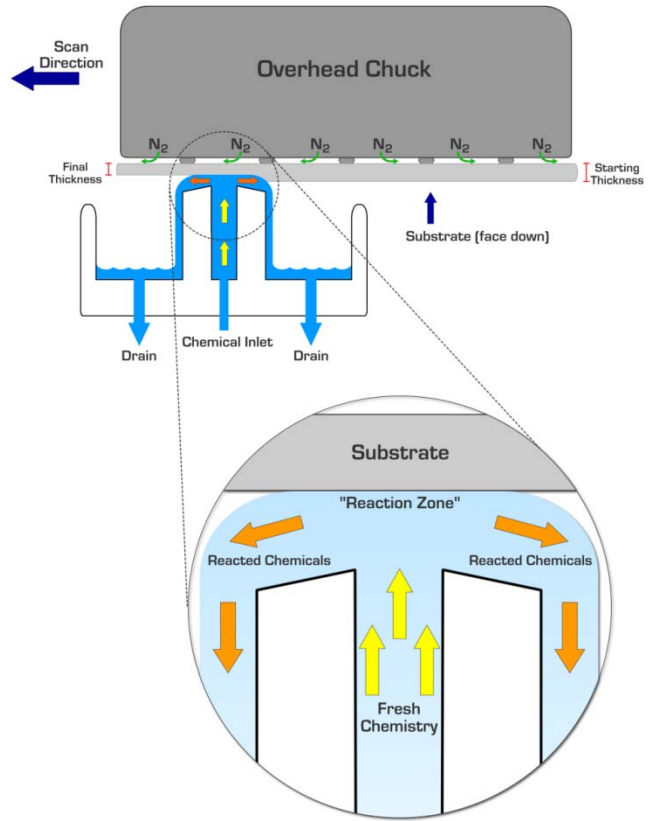
Figure 1a. Schematic representation of the LinearScan process depicting the substrate (held process side down) material being removed by the etching process, as well as the orthogonal paths of the reactants and the byproducts. The shaped flow of gas (DynamicConfinement), preventing the encroachment of fluid and vapors onto the non-process side (top), is also shown. Note the removal of material (etching) after the wafer has passed over the fluid meniscus and the different paths the reaction byproducts take to avoid interference with the supply of fresh reactants to the reaction zone.
