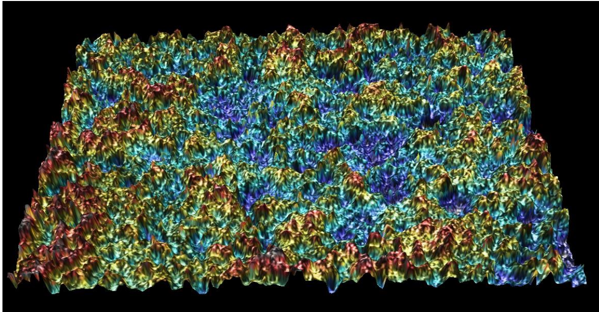
Figure 2. Confocal microscope rendered image of a LinearScan textured surface with an acidic solution viewed at 50X magnification. Note the complex and convoluted nature of the surface, and the absence of smooth flat facets. S_a=0.65\ \mu\text{m} , S_q=0.81\ \mu\text{m} , S_z=7.52\ \mu\text{m} (average, RMS, and maximum roughness depth areal parameters respectively, as per ISO 25178). Such surfaces offer an increased surface area for mechanical interlocking of deposited films, as often required in backside metallization.
