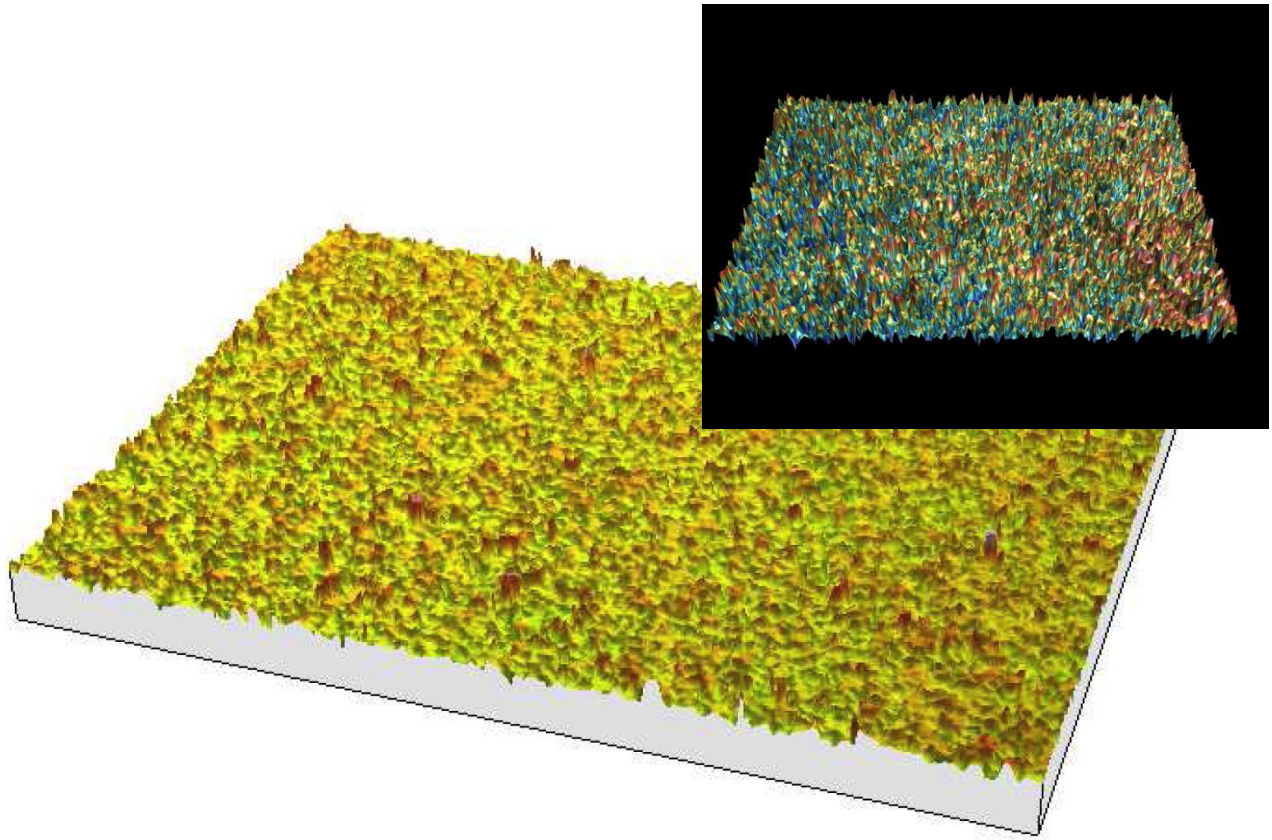
Figure 4. Acidic textures, shown in this confocal microscope image at lower magnification (20X) can be easily achieved with the LinearScan etching technology. R_a=1.82\text{ }\mu\text{m} , R_q=2.25\text{ }\mu\text{m} , R_t=13.4\text{ }\mu\text{m} , S_a=2.03\text{ }\mu\text{m} , S_q=2.62\text{ }\mu\text{m} , S_z=51.9\text{ }\mu\text{m} (average, RMS, and maximum roughness depth, line and areal parameters, respectively, as per ISO 4287 and 25178). Roughness levels achievable with this technology can range from the above to sub-micron levels. Top-right corner shows a rendering of the same X-Y-Z data.
